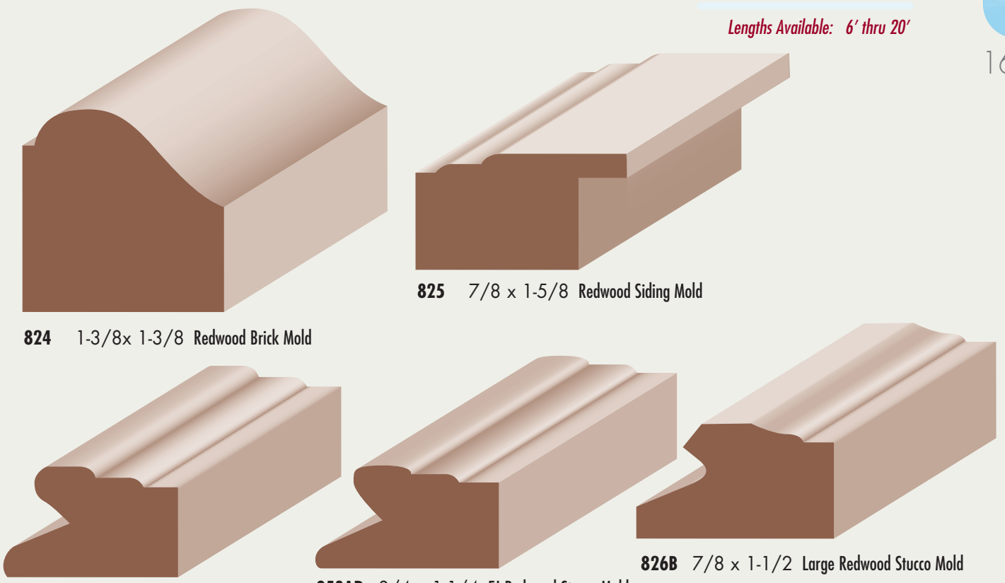
826 3/4 x 1-1/4 Redwood Stucco Mold
